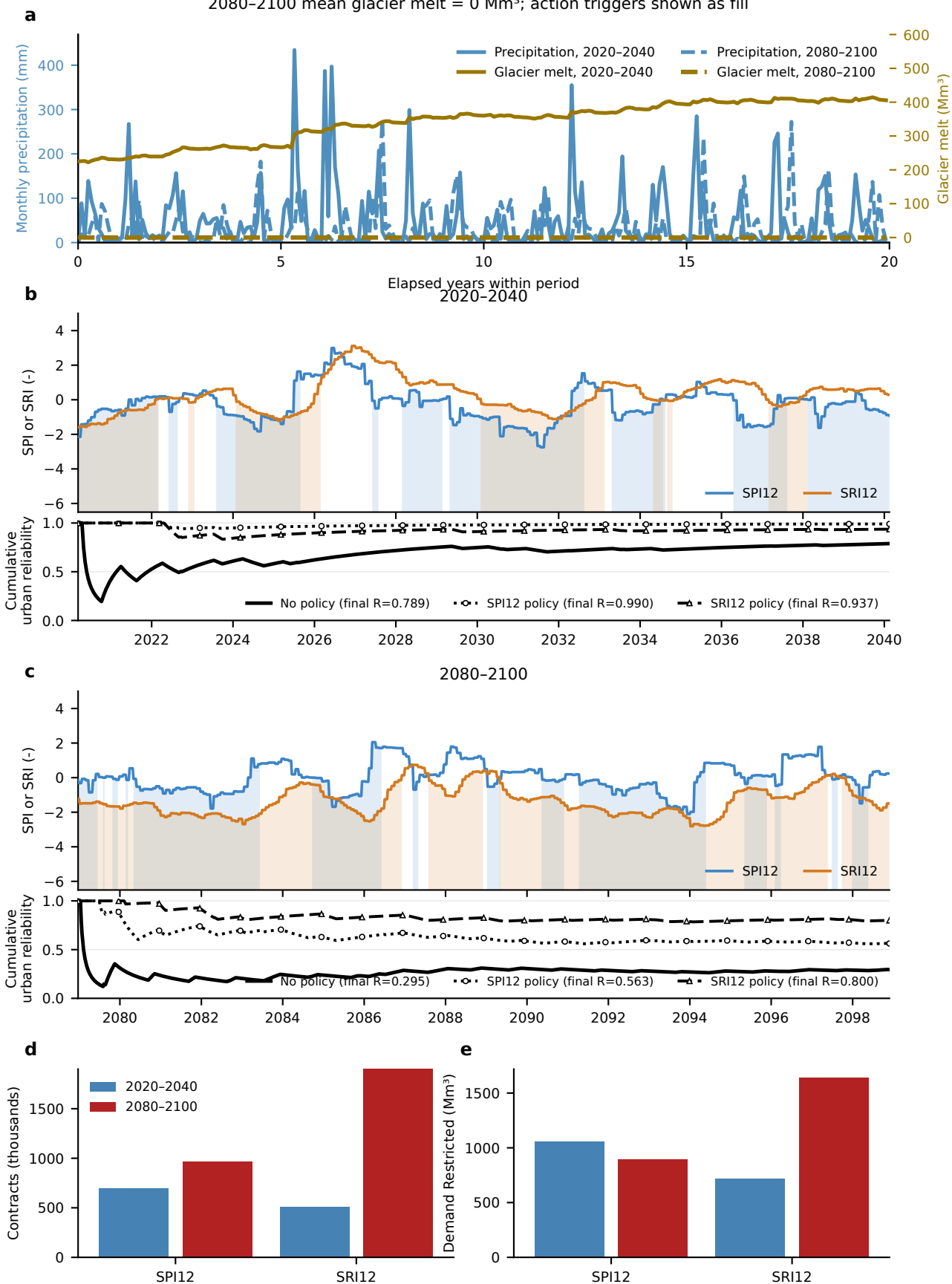
Low-glacier scenario rank 8: MIROC6_ssp585_scen02_no_drought_pert 2080–2100 mean glacier melt = 0 Mm 3 ; action triggers shown as fill
