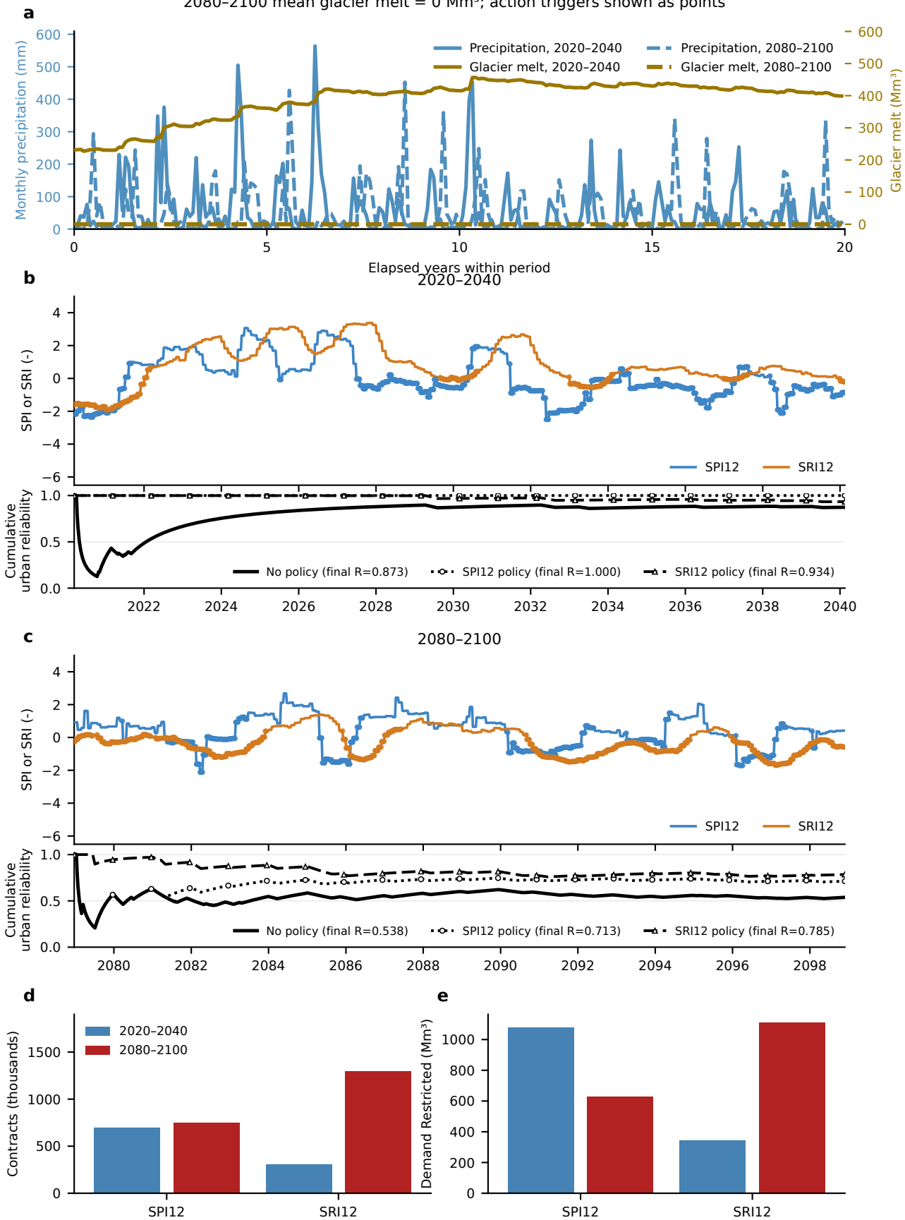
Low-glacier scenario rank 4: CNRM-CM6-1_ssp370_scen03_no_drought_pert 2080-2100 mean glacier melt = 0 Mm 3 ; action triggers shown as points
