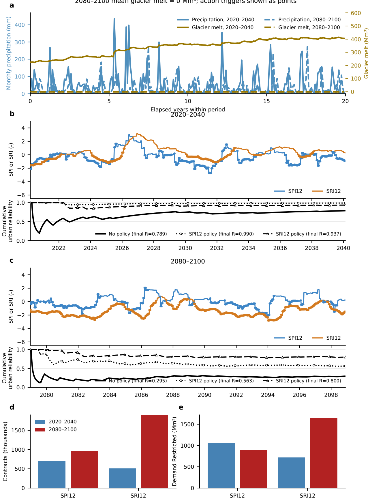
Low-glacier scenario rank 8: MIROC6_ssp585_scen02_no_drought_pert 2080-2100 mean glacier melt = 0 Mm 3 ; action triggers shown as points
