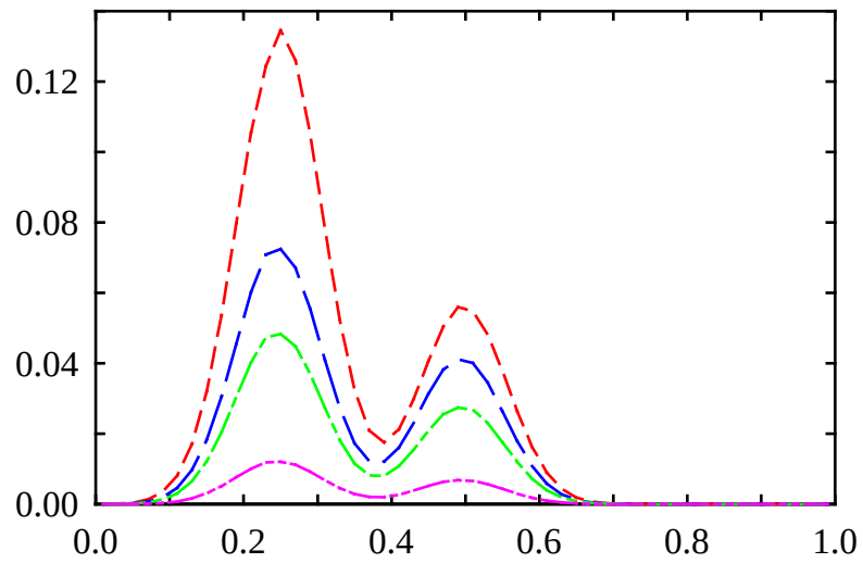
PNBIN,PNBCL [MW/m 3 ] vs r
