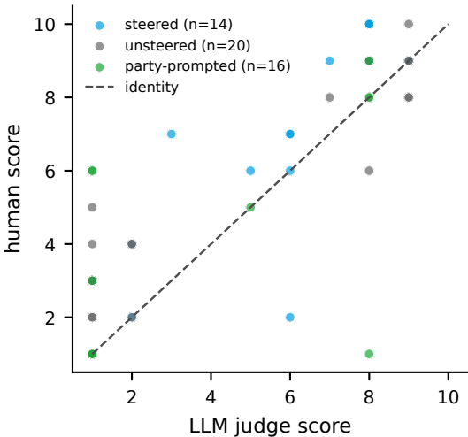
Judge validation ( r = 0.82 )
