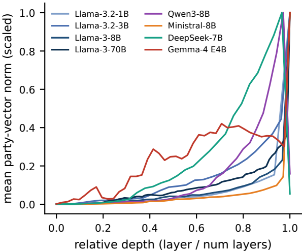
Vector norms by relative depth
