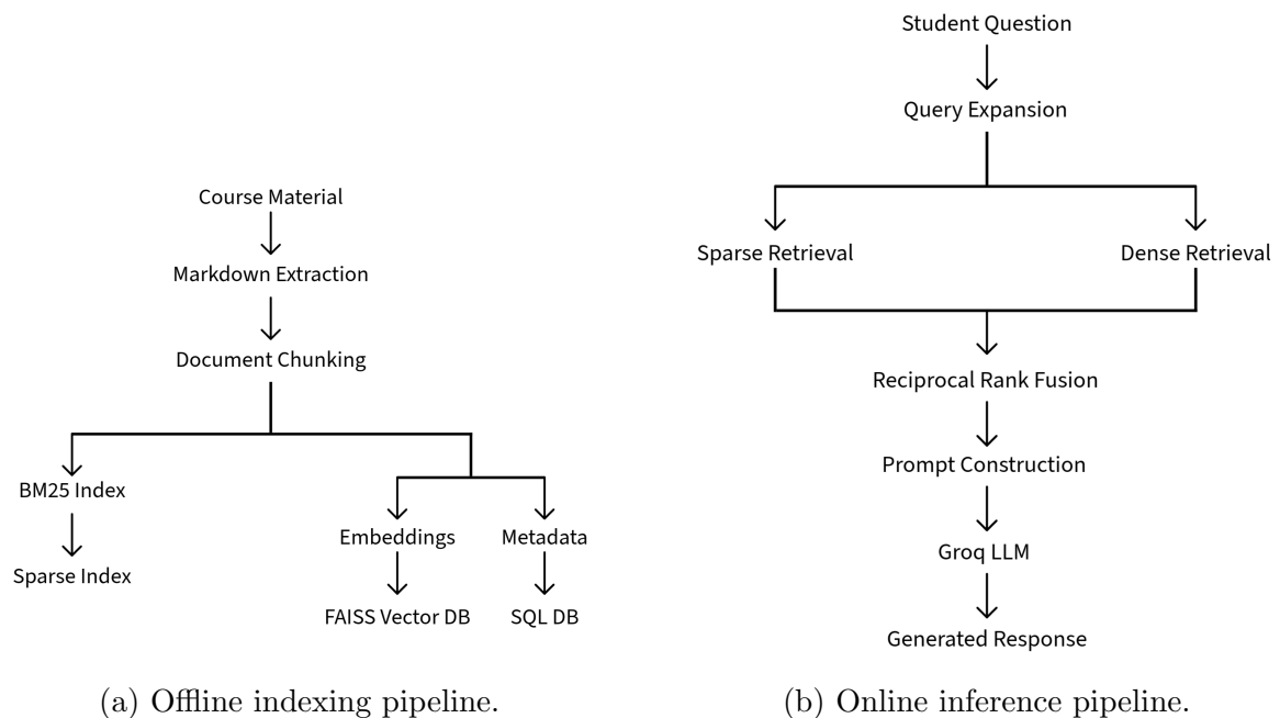
Figure 3.1: Overview of Decidr’s architecture. The offline pipeline constructs the searchable knowledge base, while the online pipeline retrieves relevant course materials and generates responses to student queries.
