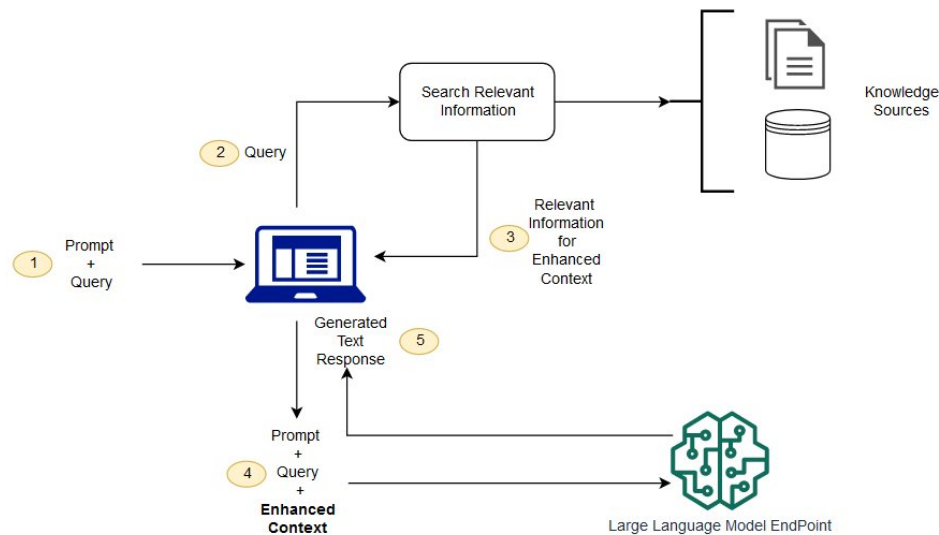
Figure 2.1: Architecture flow of Retrieval-Augmented Generation. Reprinted from [4].
