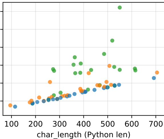
v2c / sentseq-3e4
