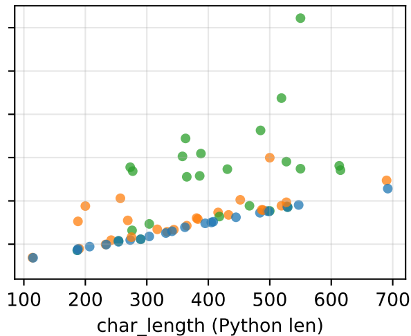
v2b / sentseq-3e4
