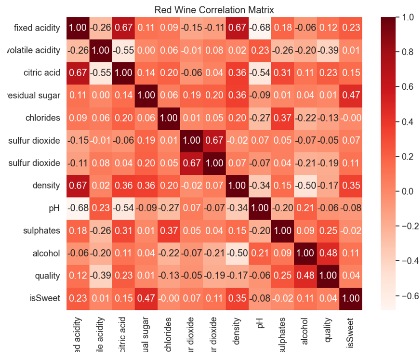
Figure 8: Correlation Matrix for Red Wine (Pearson)
