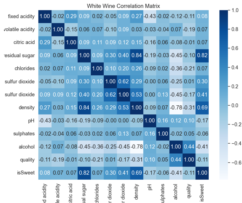
Figure 9: Correlation Matrix for White Wine (Pearson)
