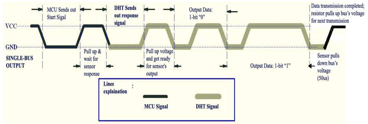
Figure 2 Overall Communication Process
