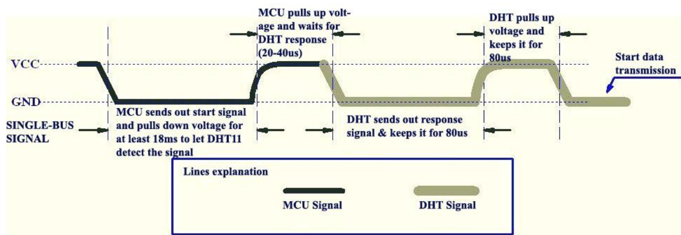
Figure 3 MCU Sends out Start Signal & DHT Responses
