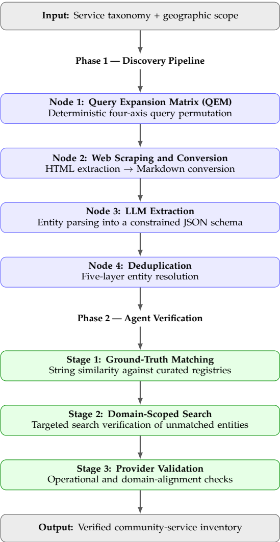
Figure 1. ARS discovery and verification pipeline adapted from thesis Figure 3.1. The vertical layout retains the full sequence of discovery, extraction, entity resolution, and evidence-verification stages.
