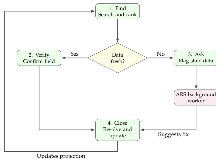
Figure 2. Pathways Find–Verify–Ask–Close flywheel adapted from thesis Figure 4.7. Human validation updates the derived projection, while stale-field requests delegate restoration to the ARS.
