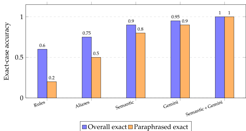
Figure 3. Study 1 exact-case accuracy for overall and paraphrased requests.
