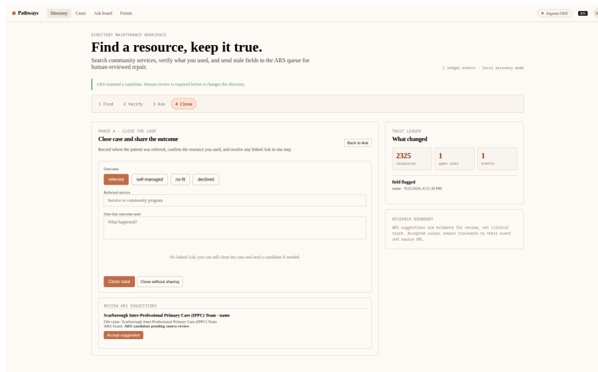
Figure 4.6: The Resolution Interface (Phase 4), enabling human operators to seamlessly validate and accept the ARS’s autonomously discovered data updates.
