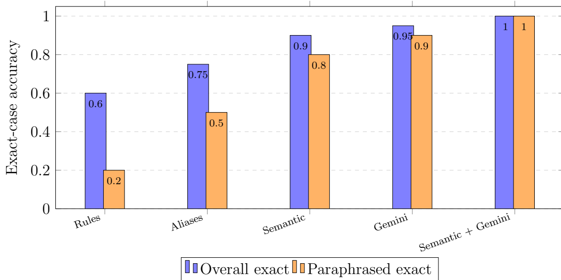
Figure 4.8: Expanded Study 1 exact-case accuracy across the five extraction conditions. Values are development-fixture results; labels are placed inside the bars.
