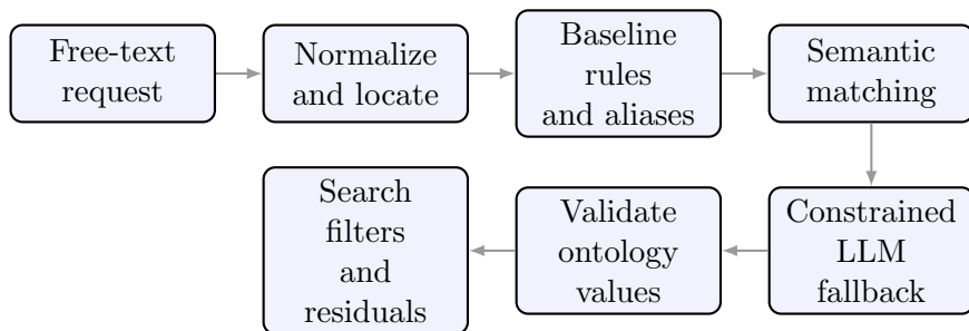
Figure 4.3: Phase 1 filter-extraction pipeline. Deterministic rules and aliases are applied first; semantic matching and the constrained LLM fallback operate only on unresolved or ambiguous residue.
