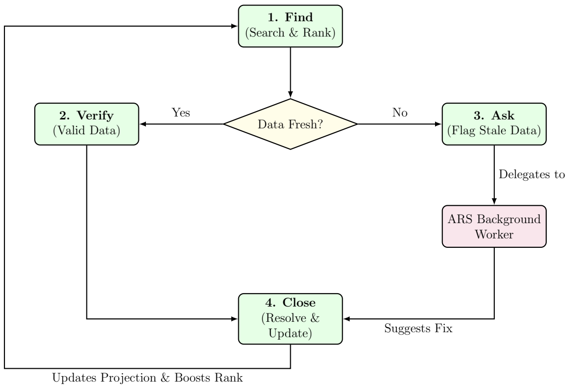
Figure 4.2: The socio-technical flywheel integrating human validation with the ARS background worker.
