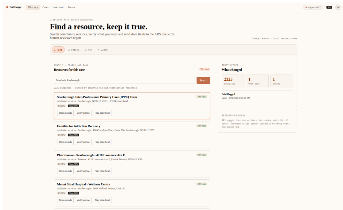
Figure 4.3: The Pathways Search Interface (Phase 1), demonstrating the explicit visual separation of algorithmic Fit Scores and temporal Trust Scores.
