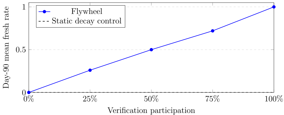
Figure 4.8: Study 3 simulated day-90 freshness as verification participation increases.
