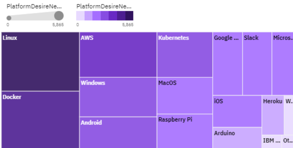
PlatformDesireNextYear
