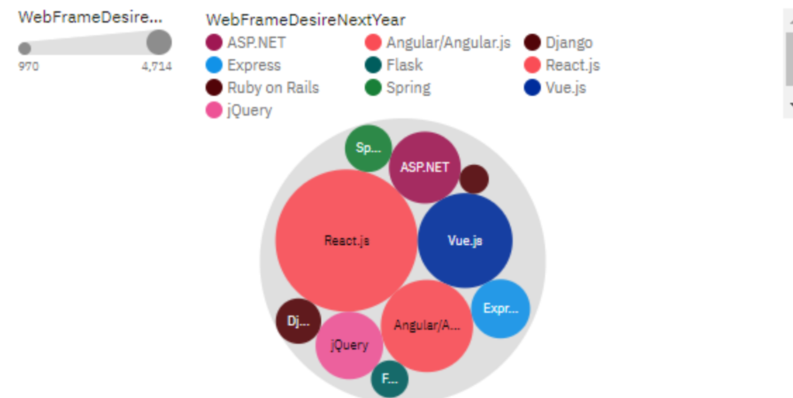
Top 10 WebFrameDesireNextYear
