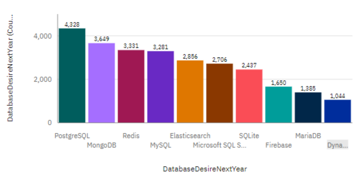
Top 10 DatabaseDesireNextYear
