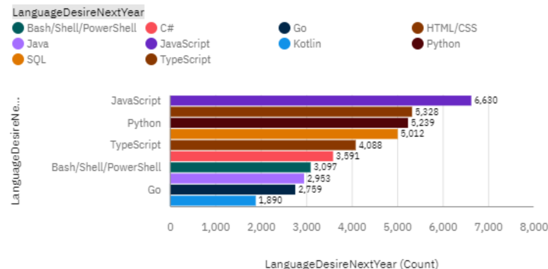
Top 10 LanguageDesireNextYear
