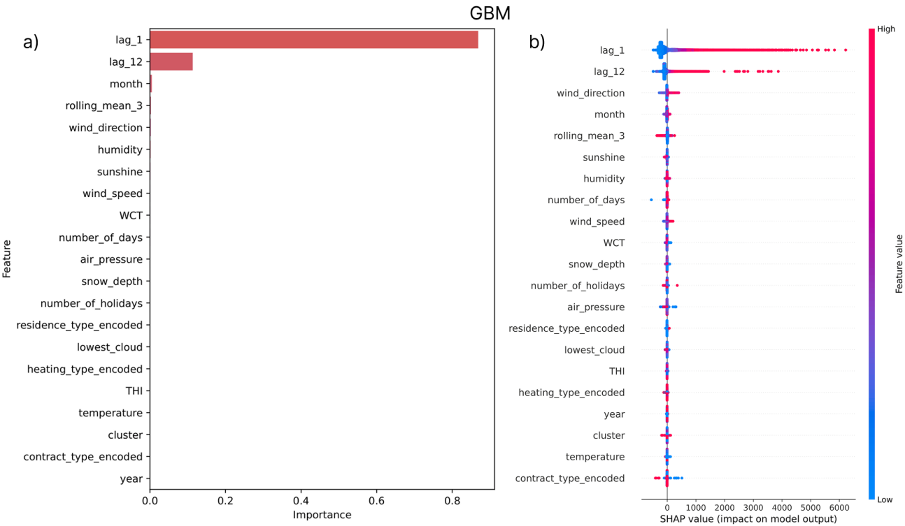
Figure 14: Feature importance (a) and SHAP summary (b) for GBM.
