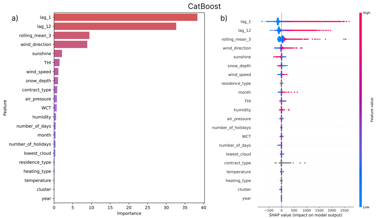
Figure 17: Feature importance (a) and SHAP summary (b) for CatBoost.
