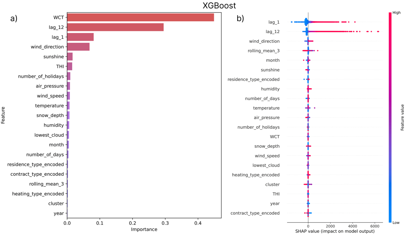
Figure 15: Feature importance (a) and SHAP summary (b) for XGBoost.
