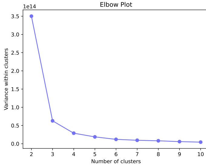
Figure 6: Elbow plot for finding the optimal number of household consumption profile clusters k .
