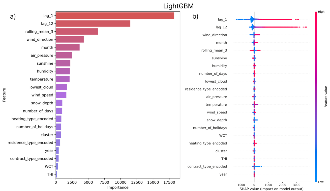
Figure 16: Feature importance (a) and SHAP summary (b) for LightGBM.
