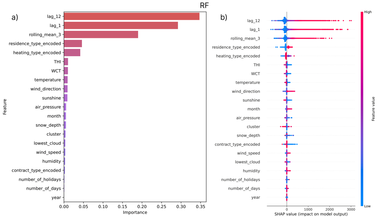
Figure 13: Feature importance (a) and SHAP summary (b) for RF.
