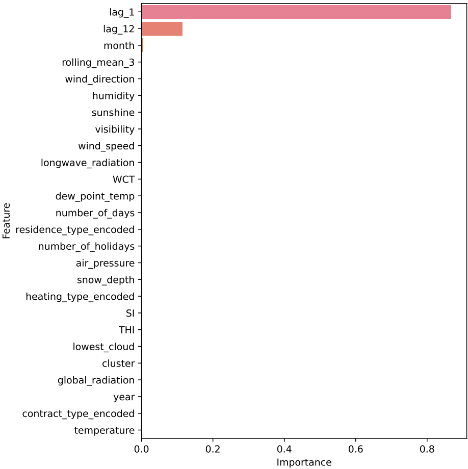
Figure 12: Feature importances for GBM.
