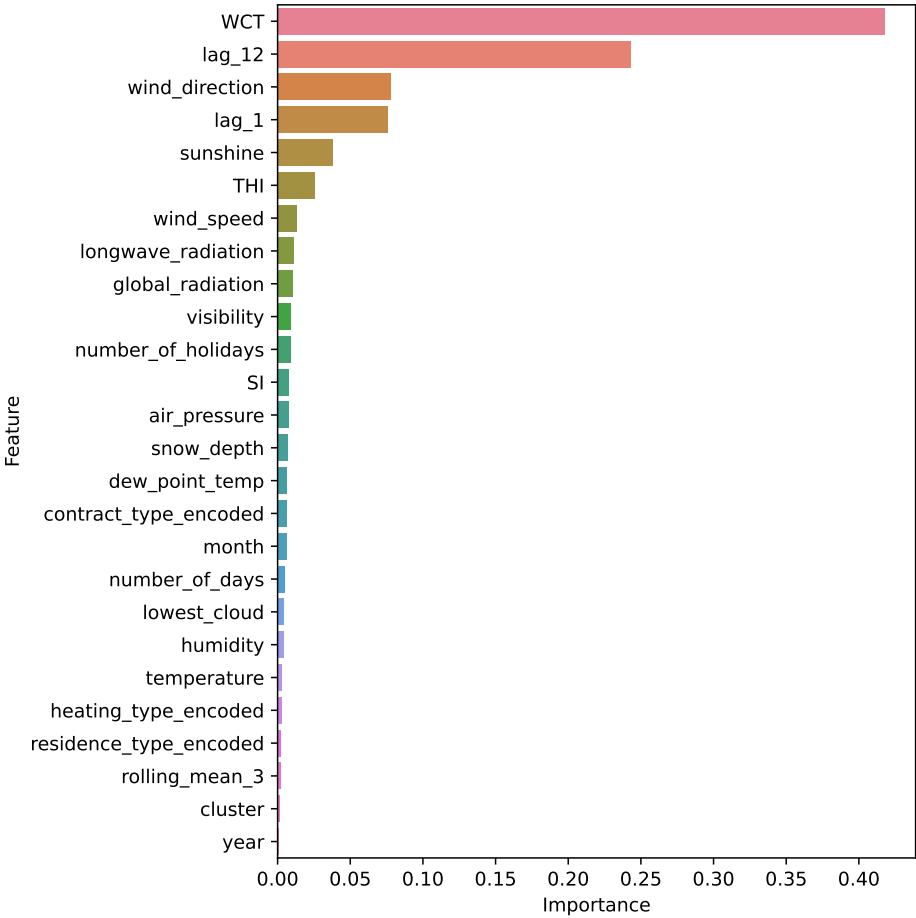
Figure 13: Feature importances for XGBoost.
