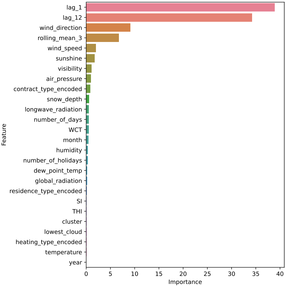
Figure 15: Feature importances for CatBoost.
