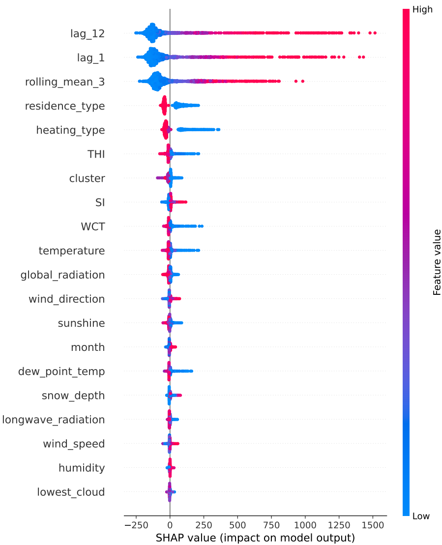
Figure 16: SHAP summary for RF.
