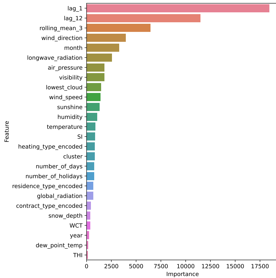
Figure 14: Feature importances for LightGBM.
