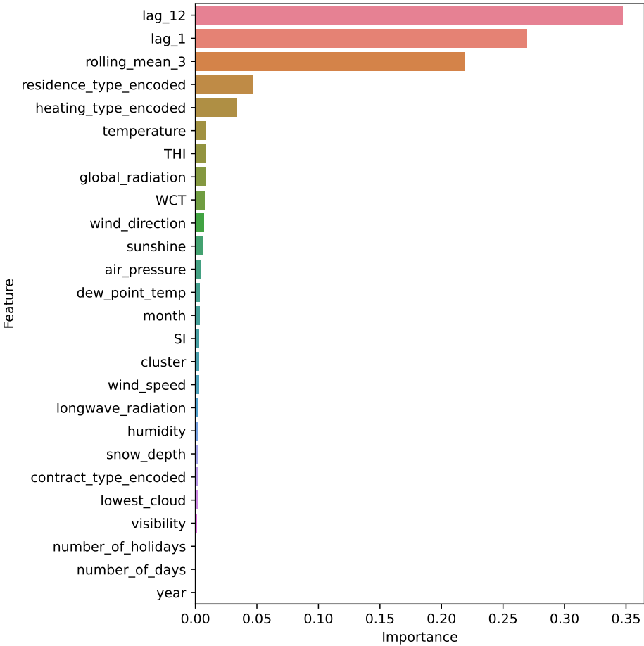
Figure 11: Feature importances for RF.
