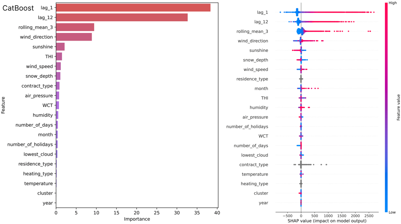
Figure 17: Feature importance and SHAP summary for CatBoost.
