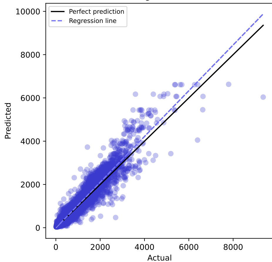
LightGBM
