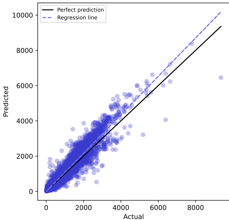
XGBoost
