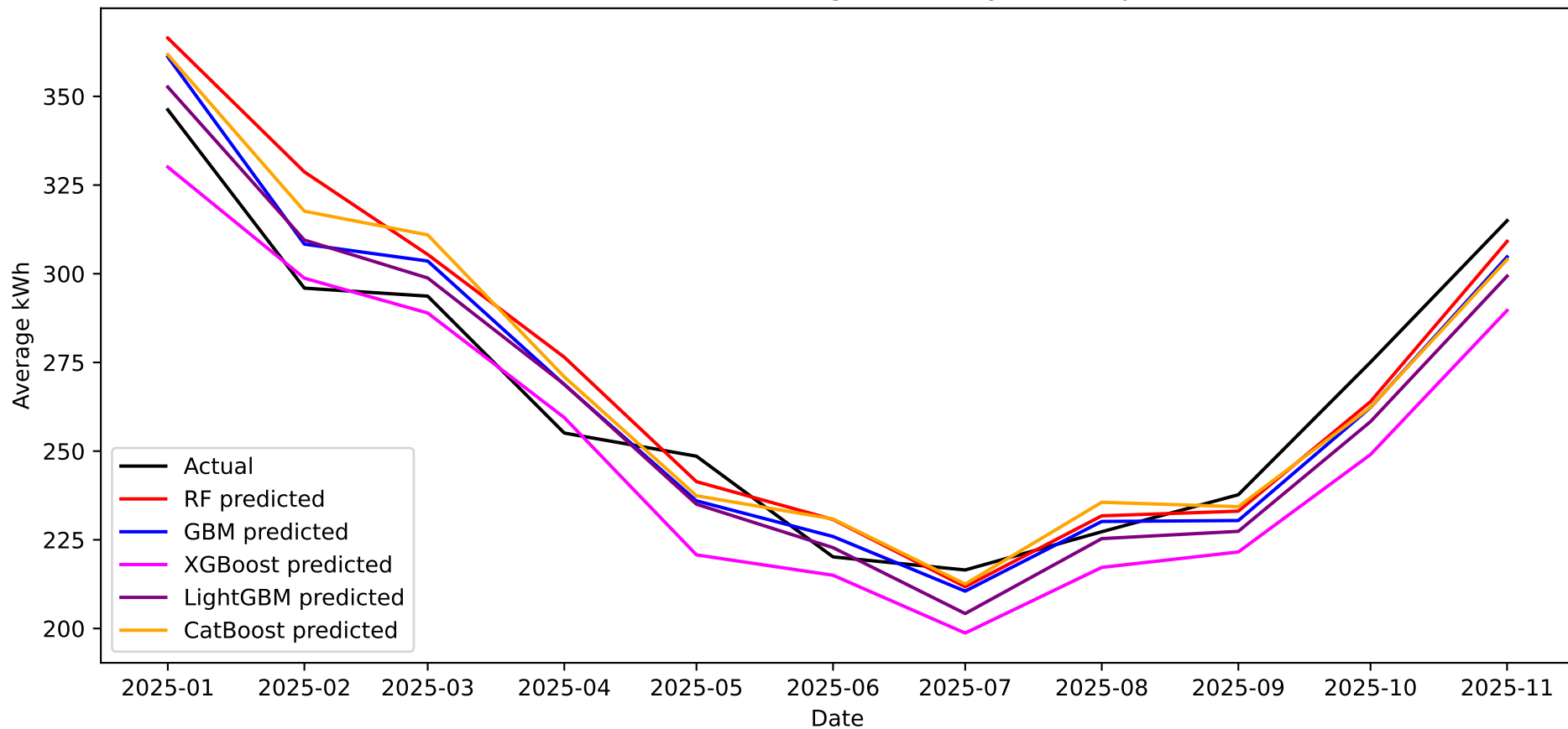
Actual vs Predicted Average Electricity Consumption
