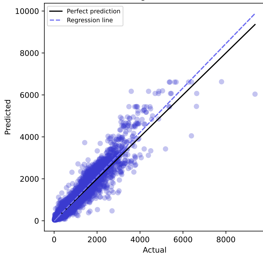
LightGBM
