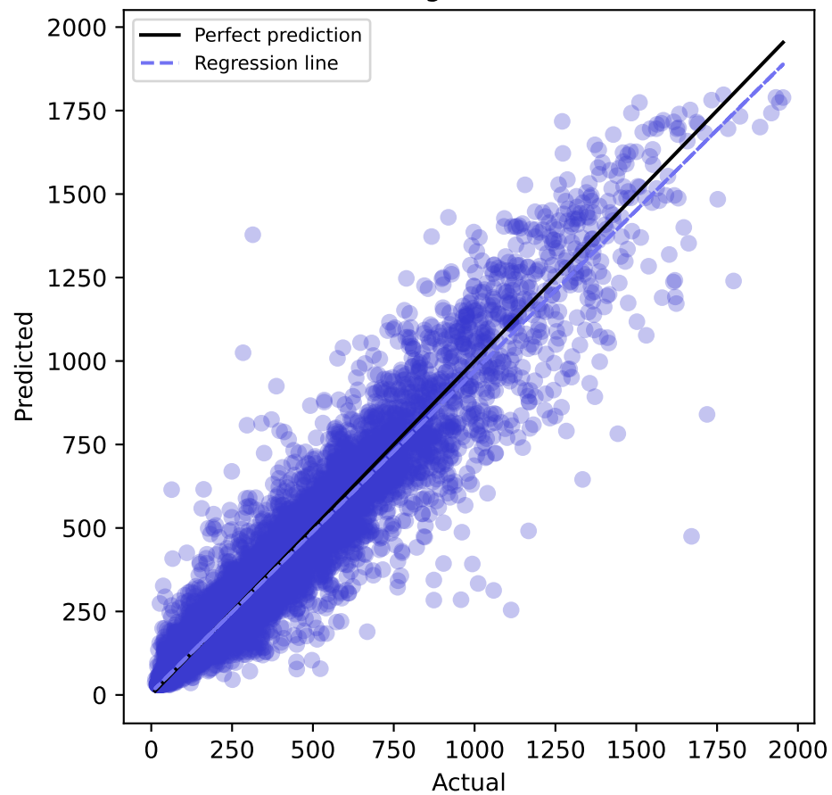
LightGBM
