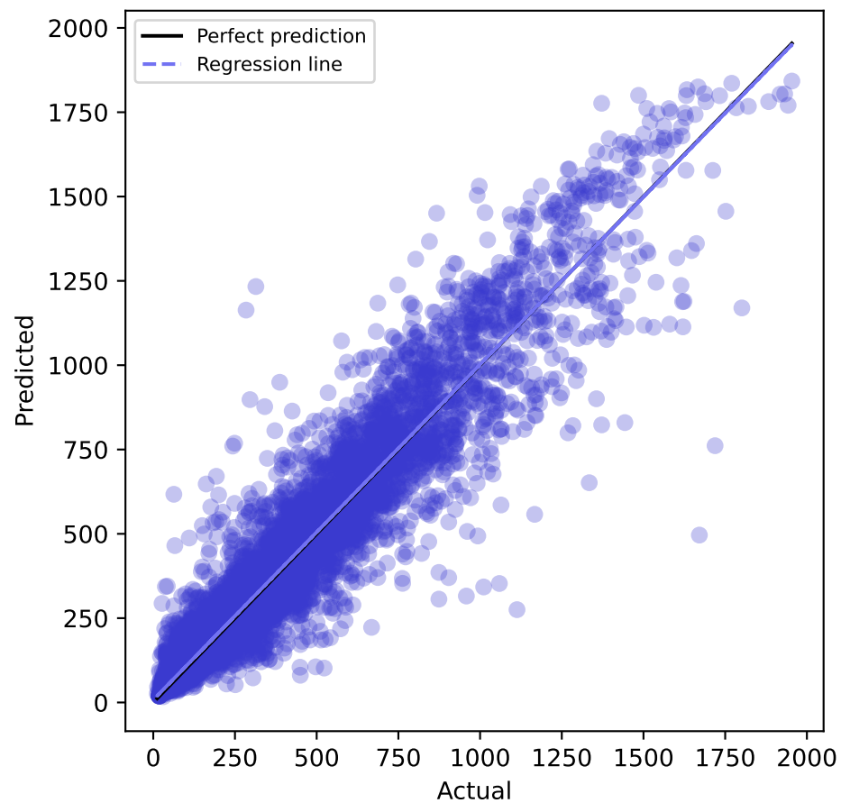
XGBoost
