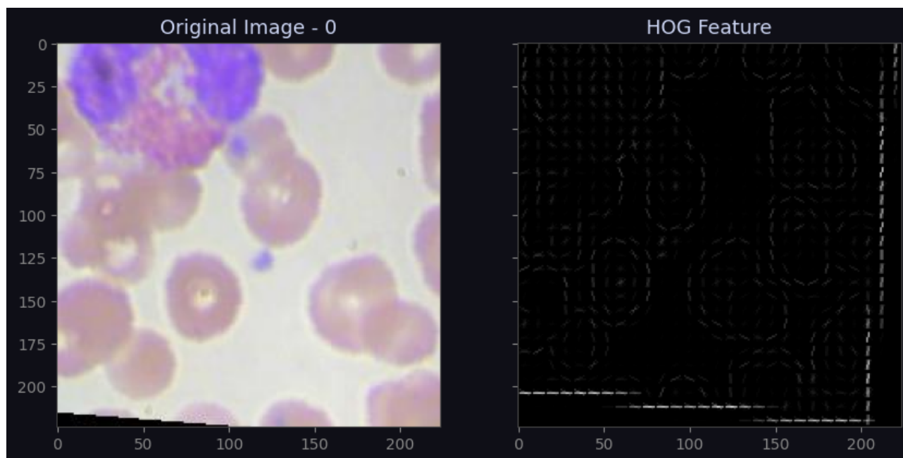
Figure 1: Illustrative HOG feature
