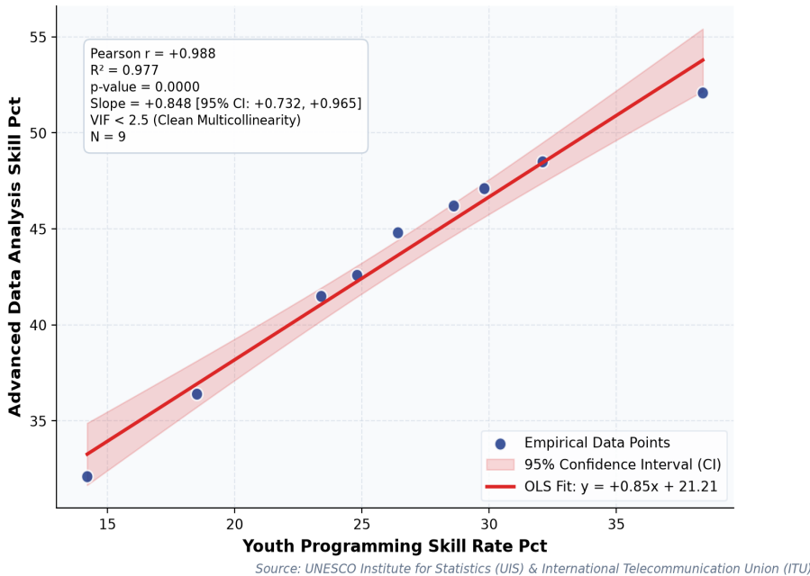
Figure 2: Empirical Quantitative Trajectory & Relational Fit for unesco_world_ict_skills .
