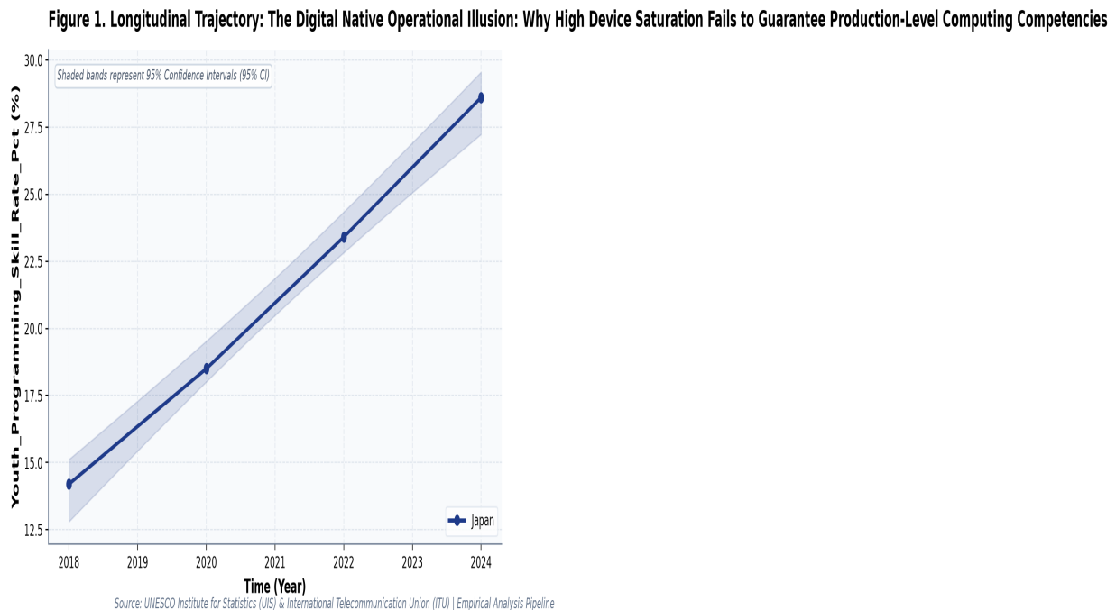
Figure 1: Empirical Quantitative Trajectory & Relational Fit for unesco_world_ict_skills .
