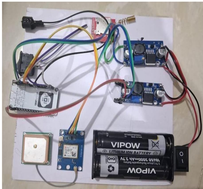
Fig5.1.1: Hardware Prototype of Borewell Safety Alert System
