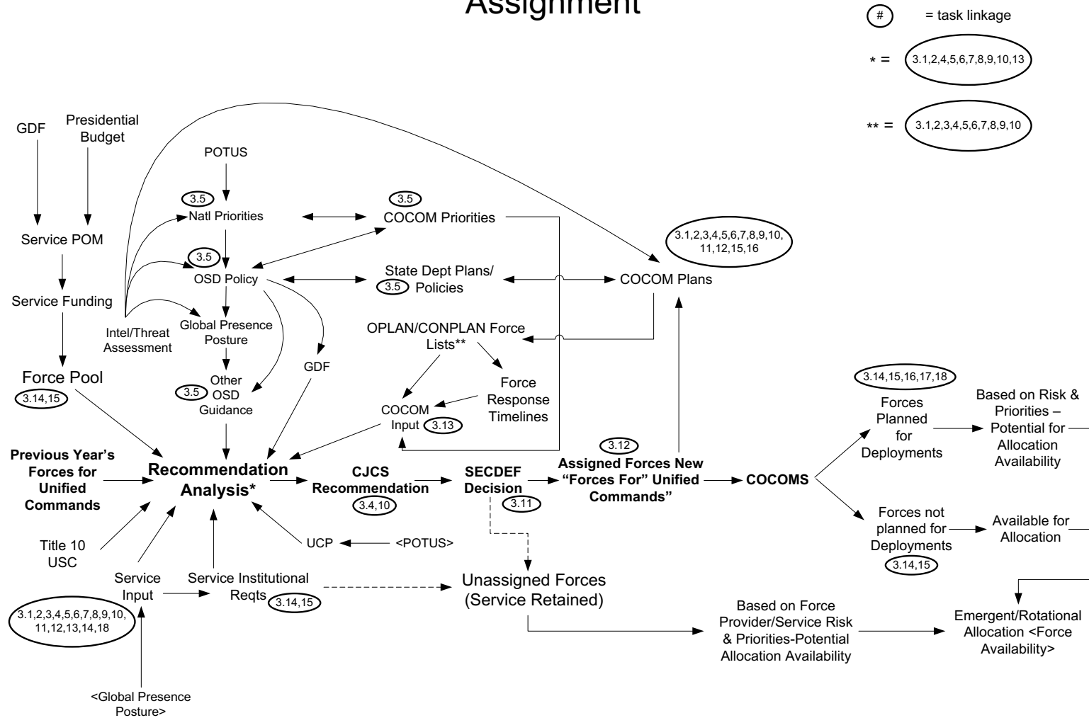
Figure H-1 GFM Process Modeling, Assignment, with Task Linkage
