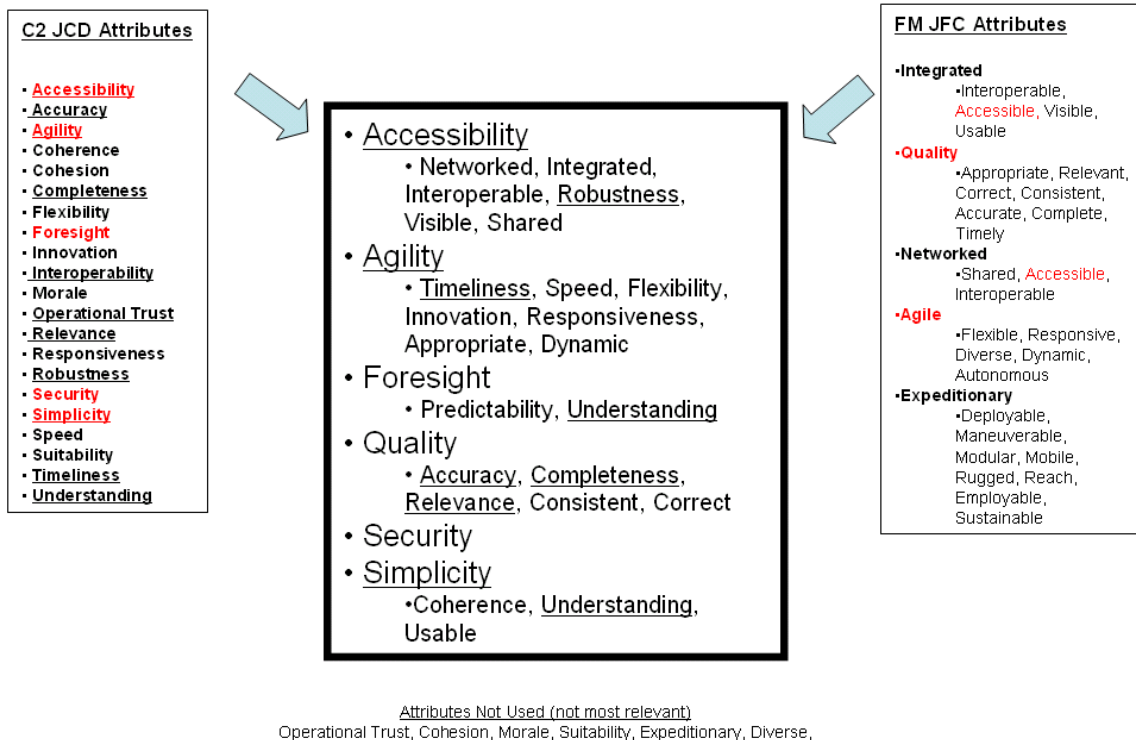
Figure D-4-1 Pedigree of GFM Attributes
