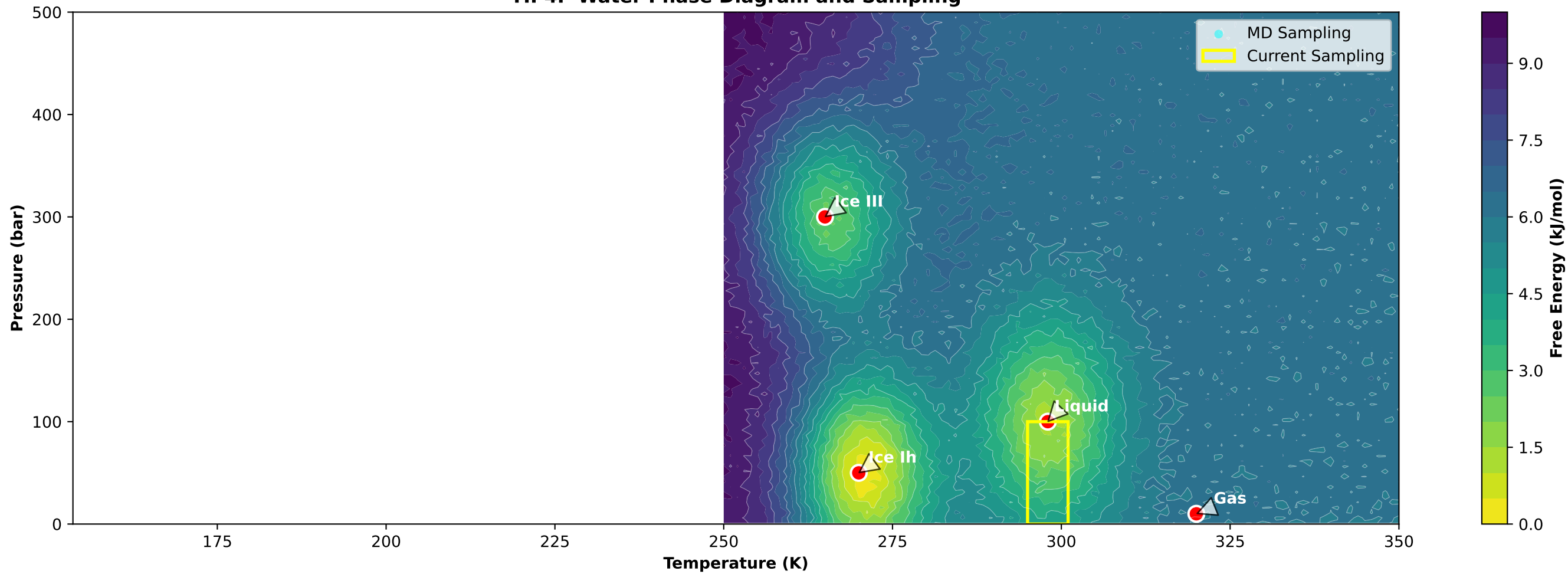
TIP4P Simulation at 298K - Actual Energy Data
