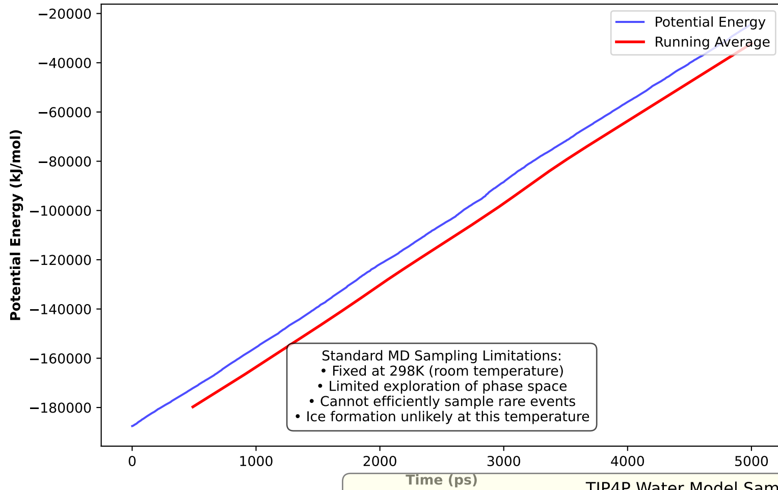
TIP4P Simulation at 298K - Actual Energy Data
