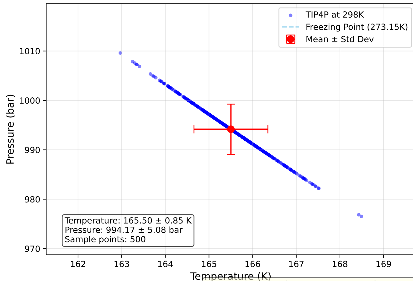
Current TIP4P Simulation at 298K
