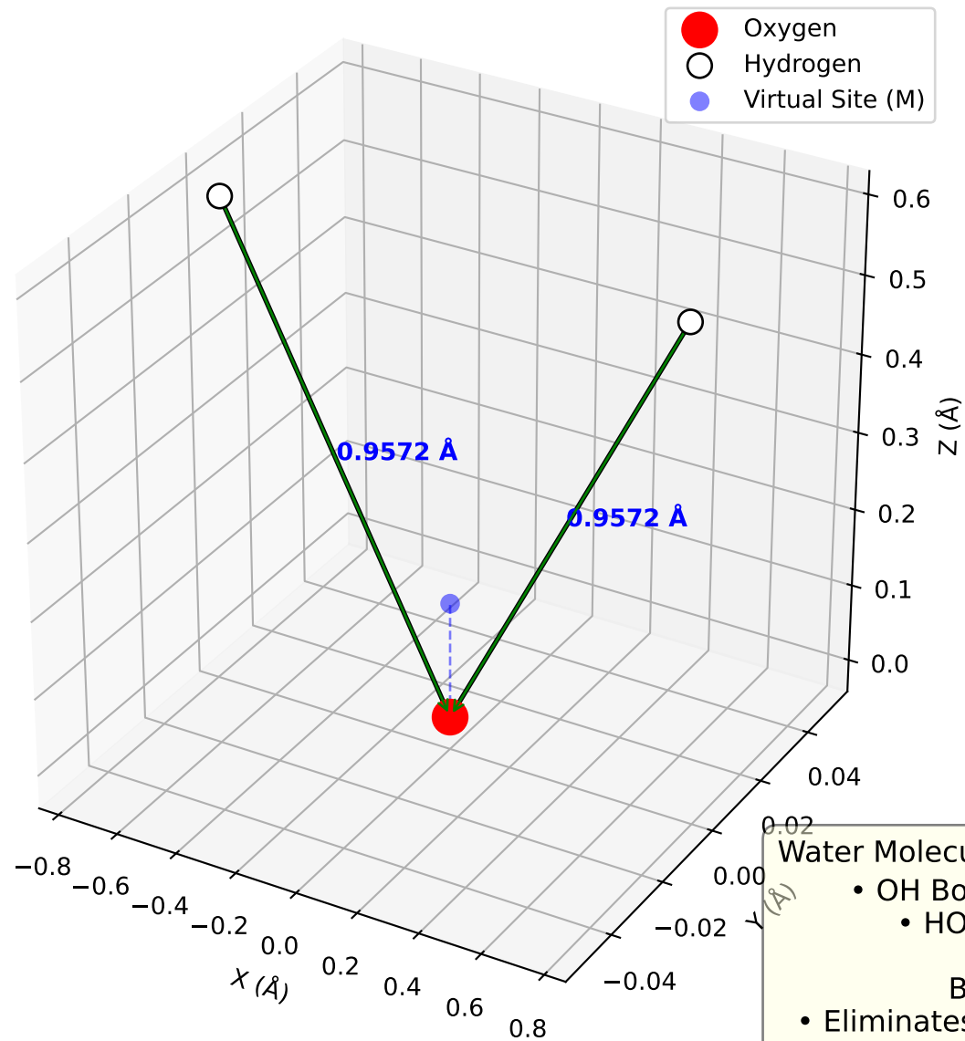
3D Water Molecule with Constraints
