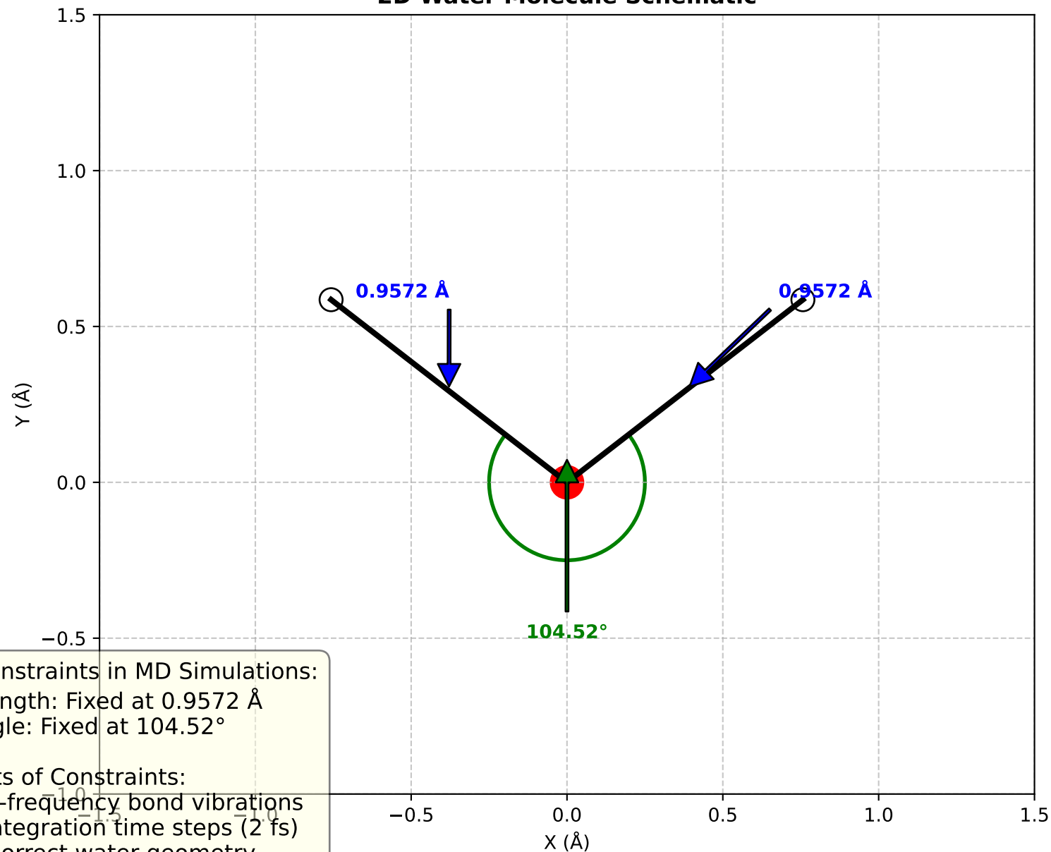
2D Water Molecule Schematic
