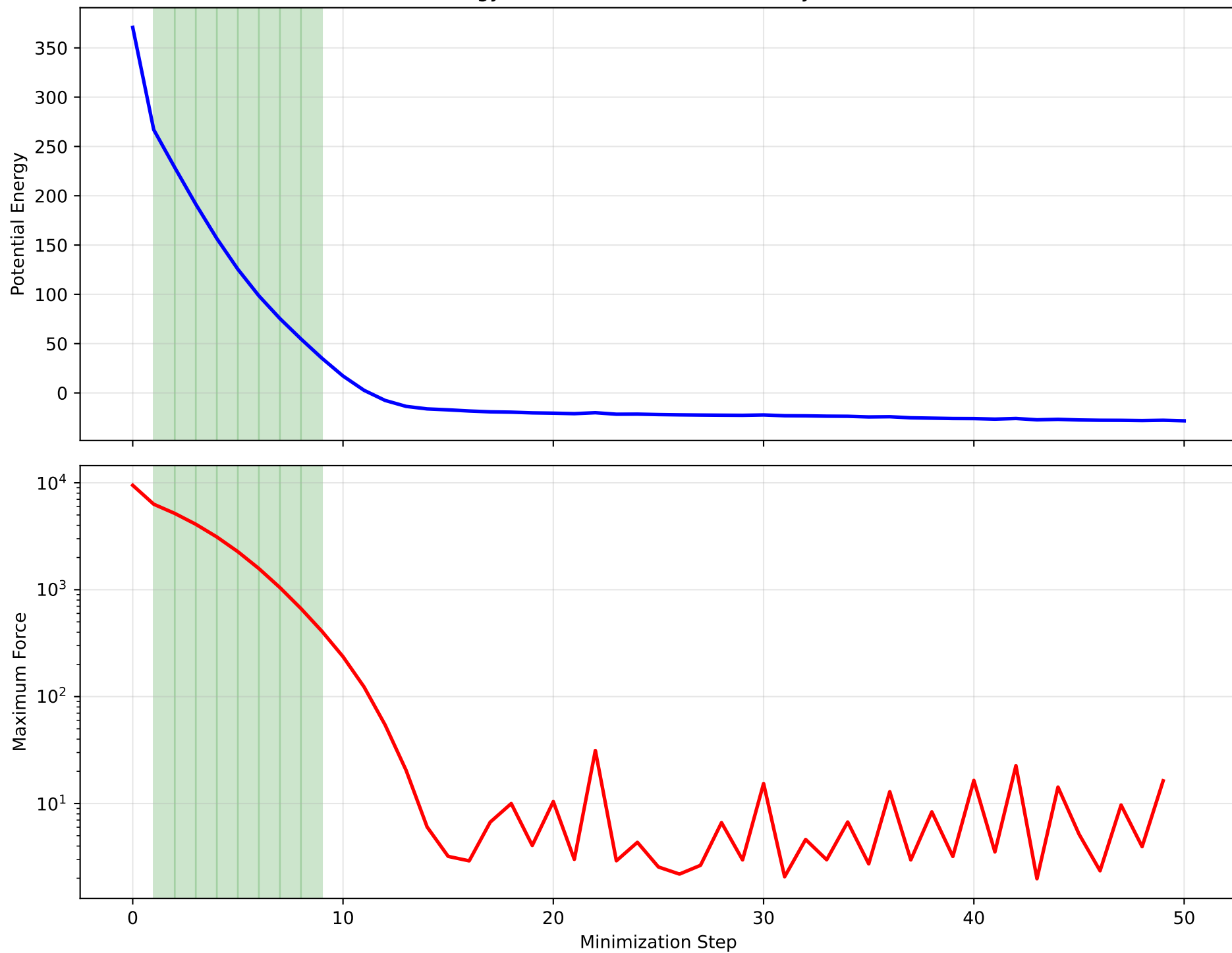
Energy Minimization in Molecular Dynamics
