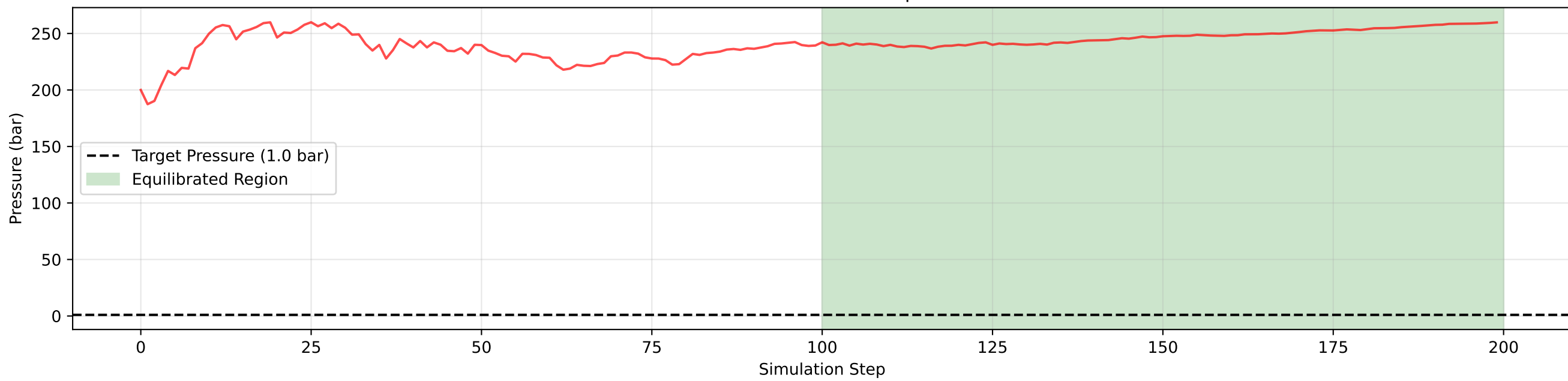
Barostat Action: Volume Adjustment
