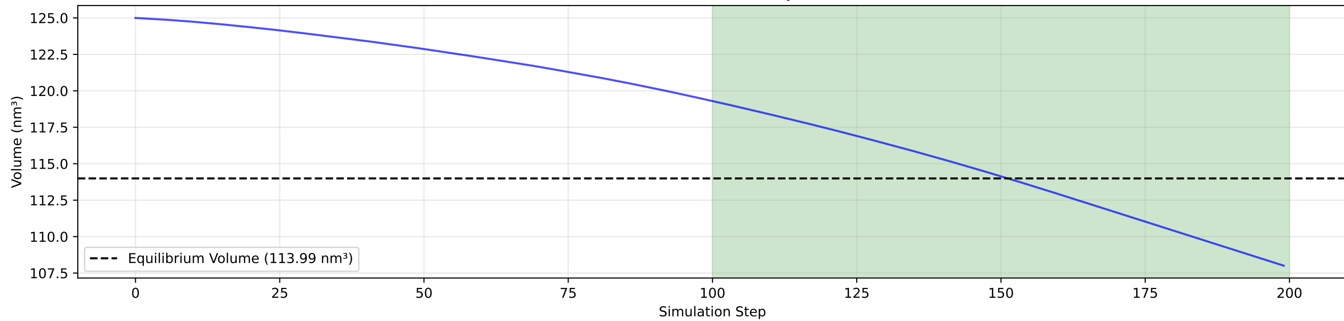
Simulation Box Evolution During NPT Equilibration
