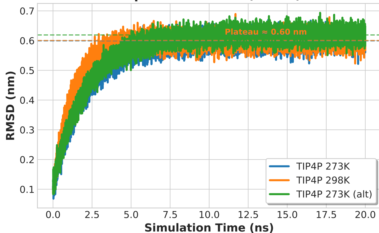
Root Mean Square Deviation (RMSD) Over Time
