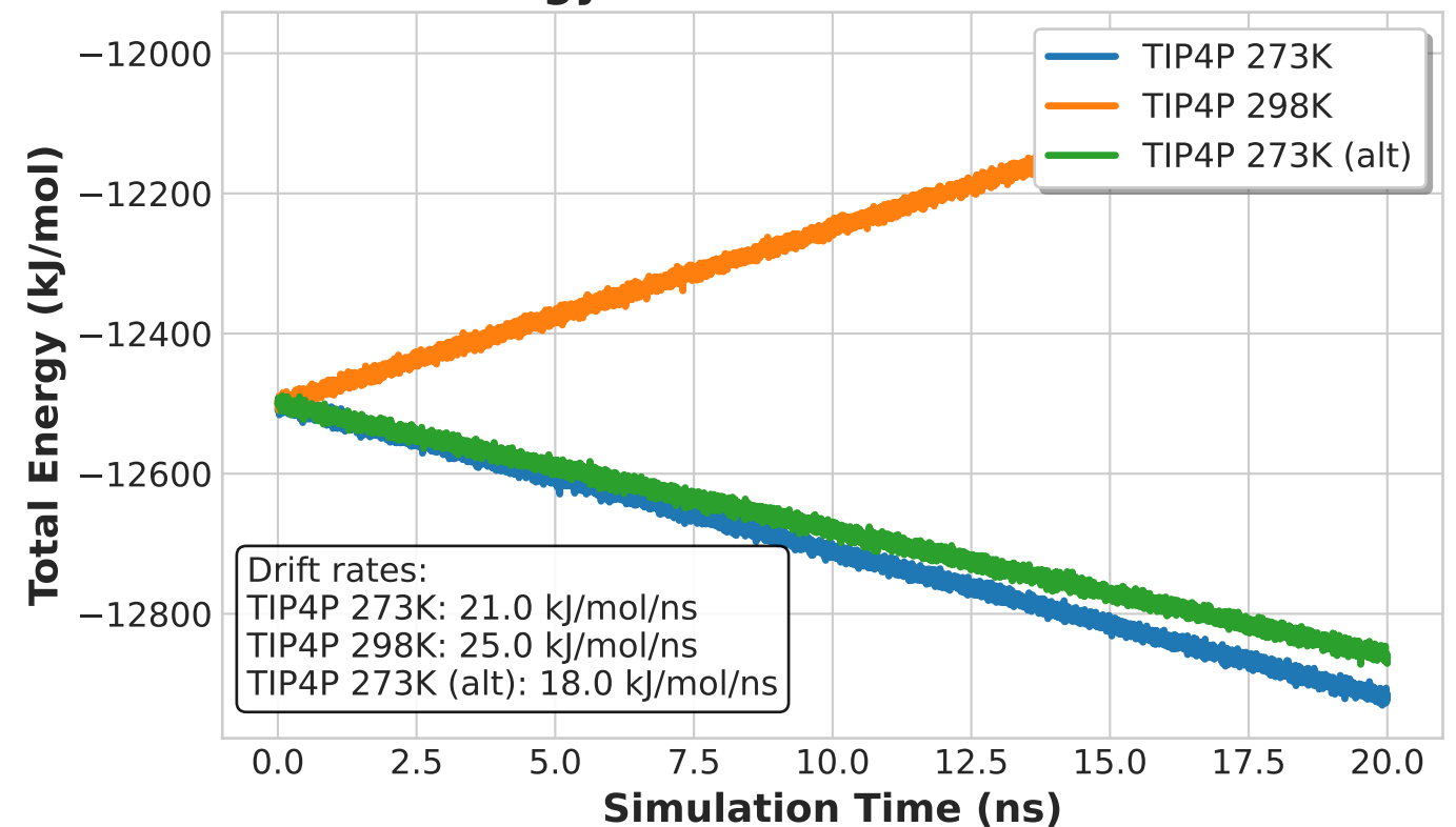
Energy Drift in Different Models
