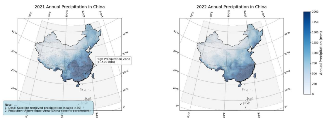
Annual Precipitation Distribution in China (2021 vs 2022)
