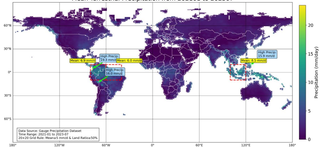
Mean Terrestrial Precipitation from 202101 to 202307
