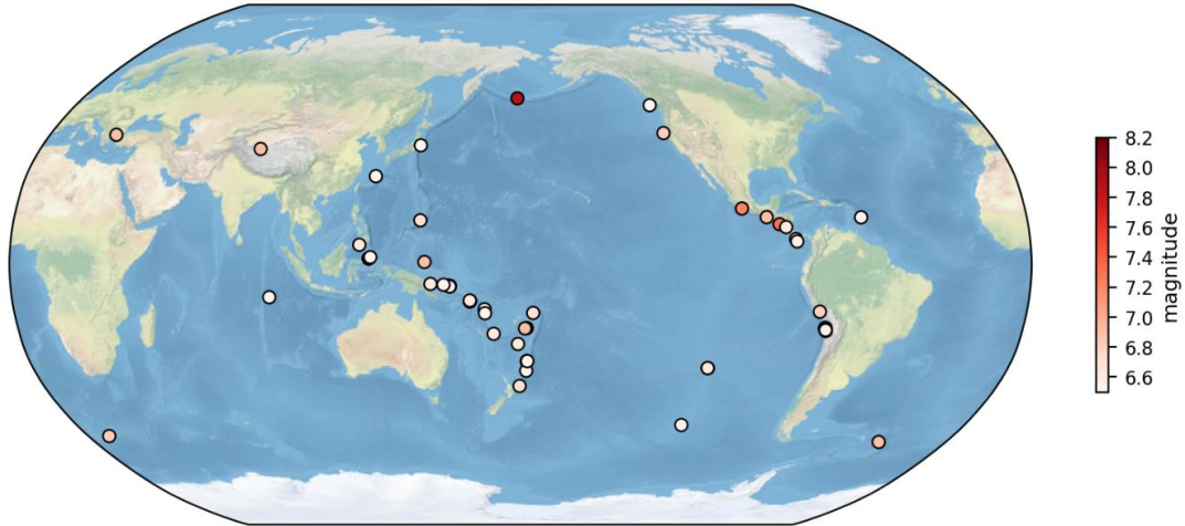
Top 50 Earthquakes of 2014
