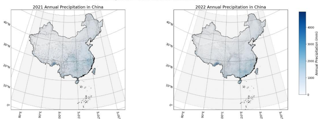
Annual Precipitation Distribution in China (2021 vs 2022)
