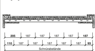
Ortgang - Detail
