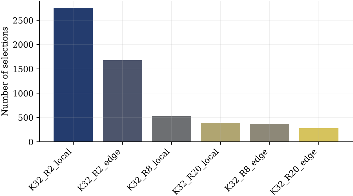
PIR-Contextual-Bandit (LinUCB): learned arm allocation (summed over 5 seeds)
