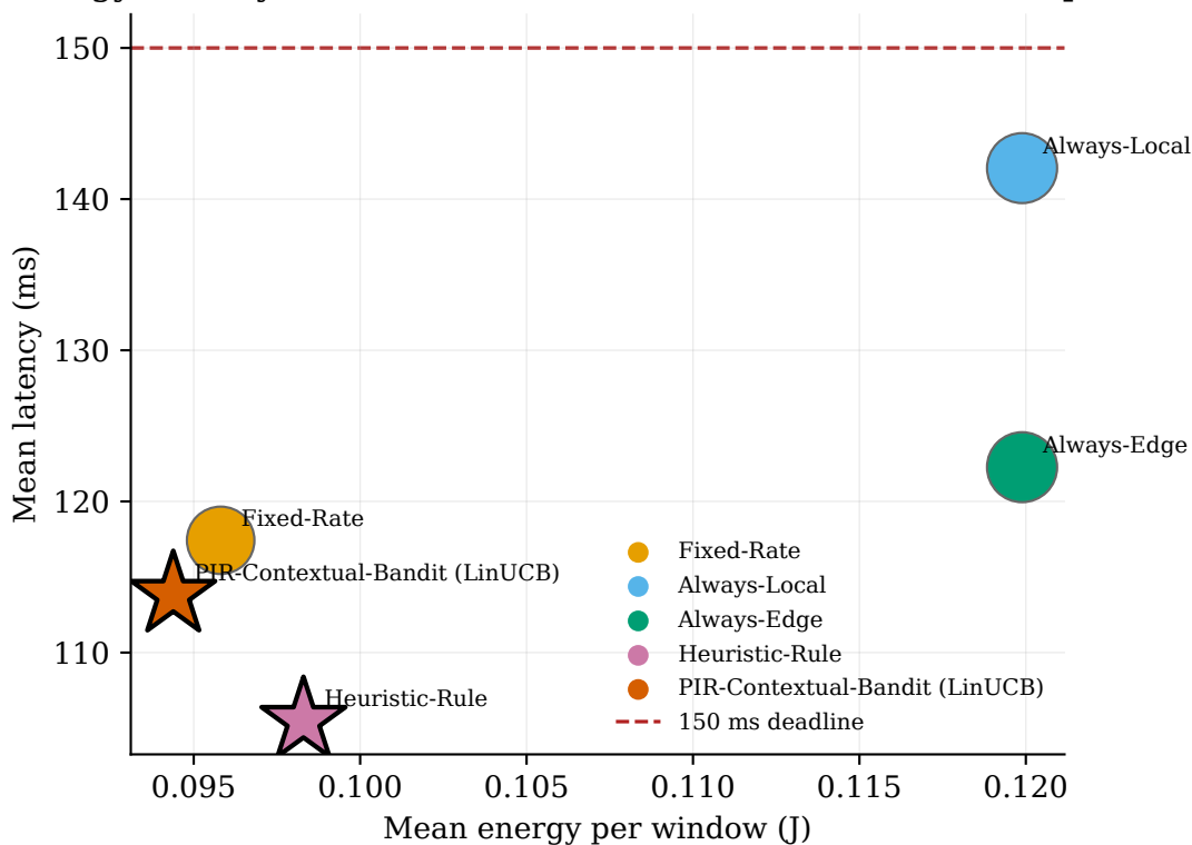
Energy-latency tradeoff (marker size \propto PDR; \star = Pareto-optimal)
