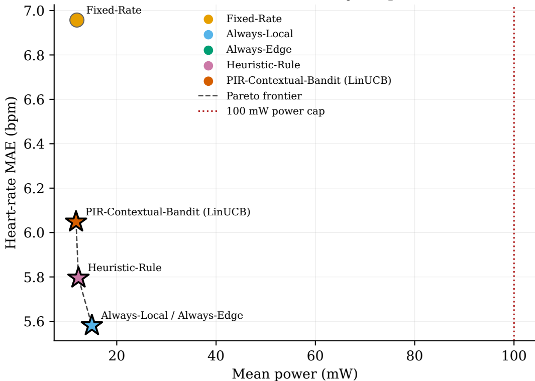
Pareto frontier: accuracy vs. power
