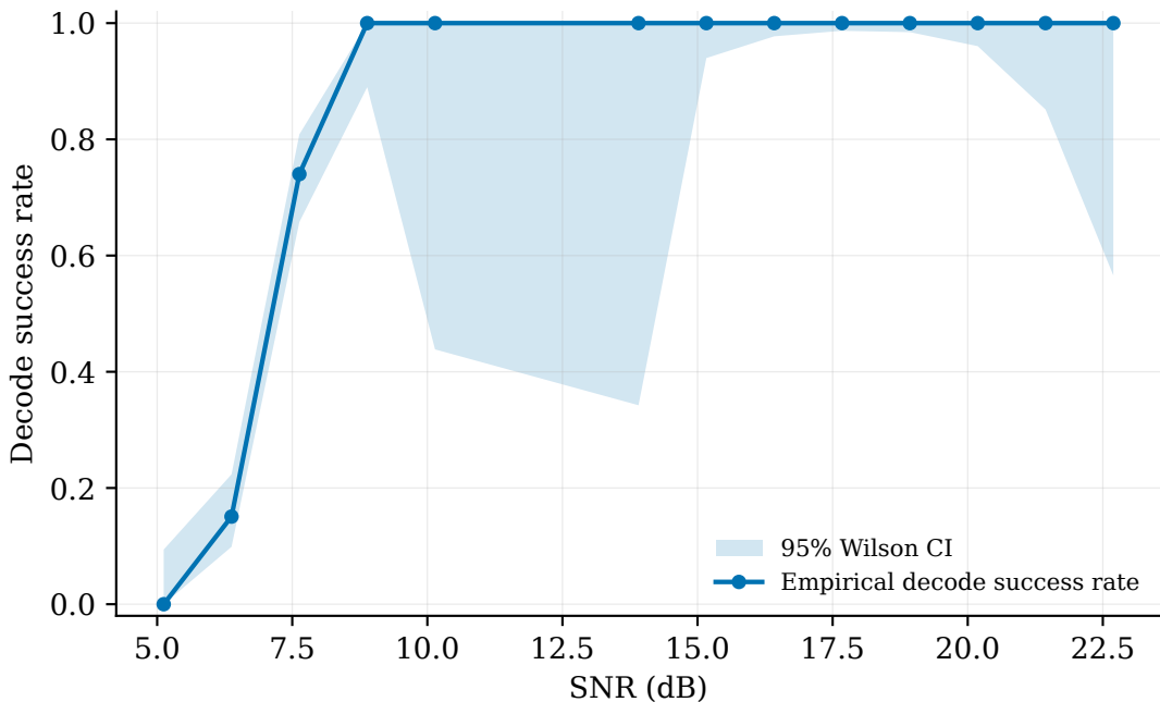
Decode success vs. channel SNR
