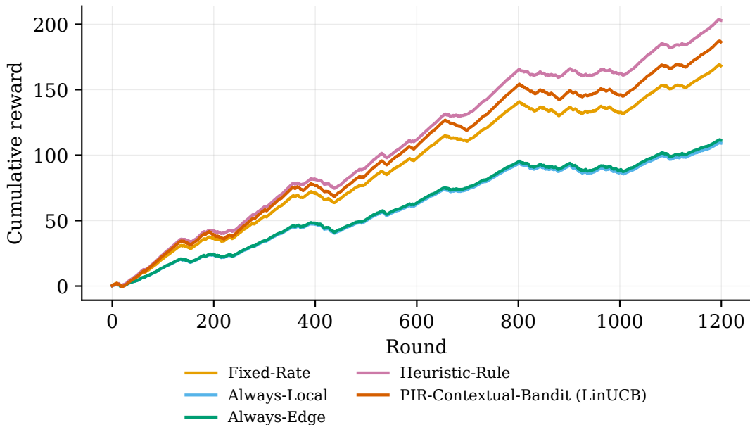
Cumulative reward
