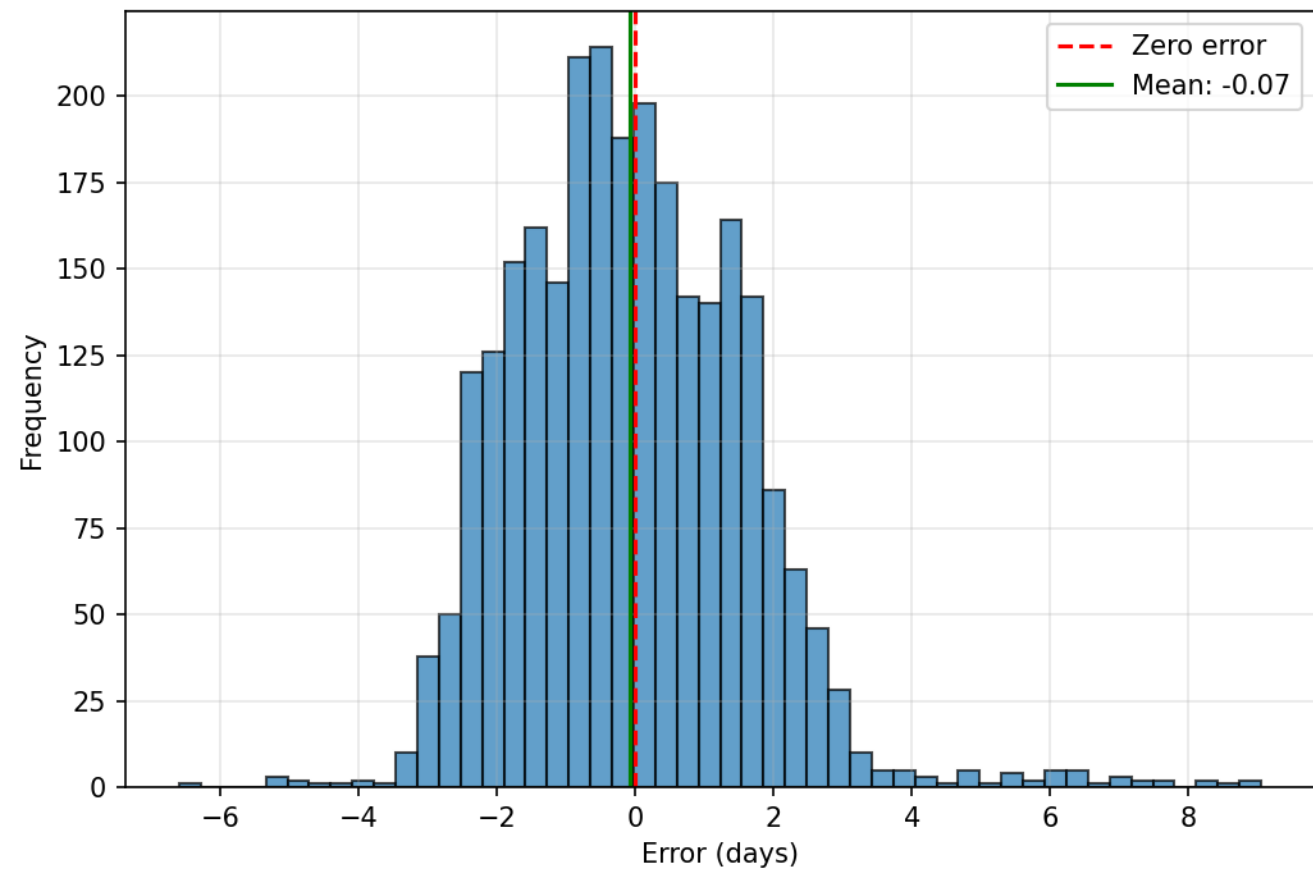
Error Distribution
