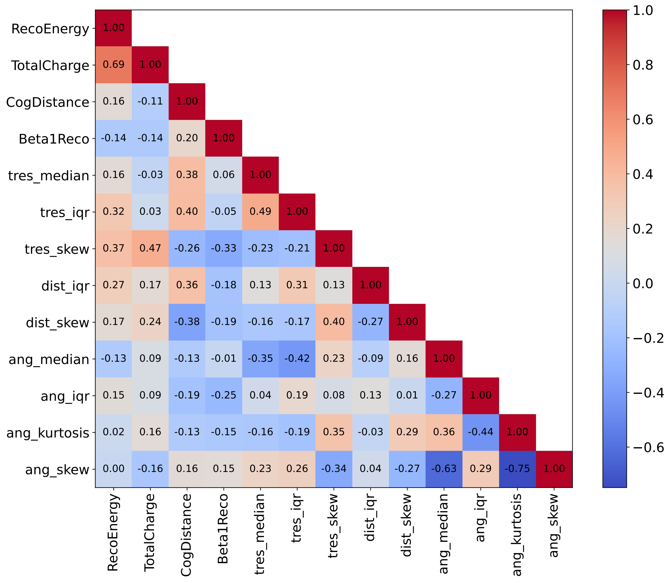
Correlation Matrix Hadronic Showers
