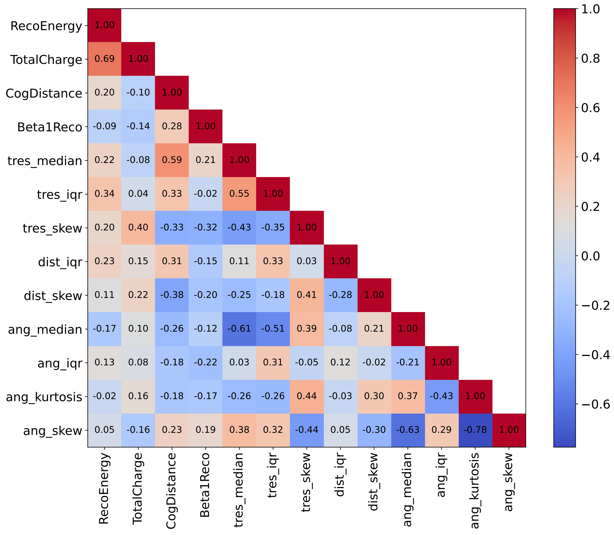
Correlation Matrix \nu_\mu
