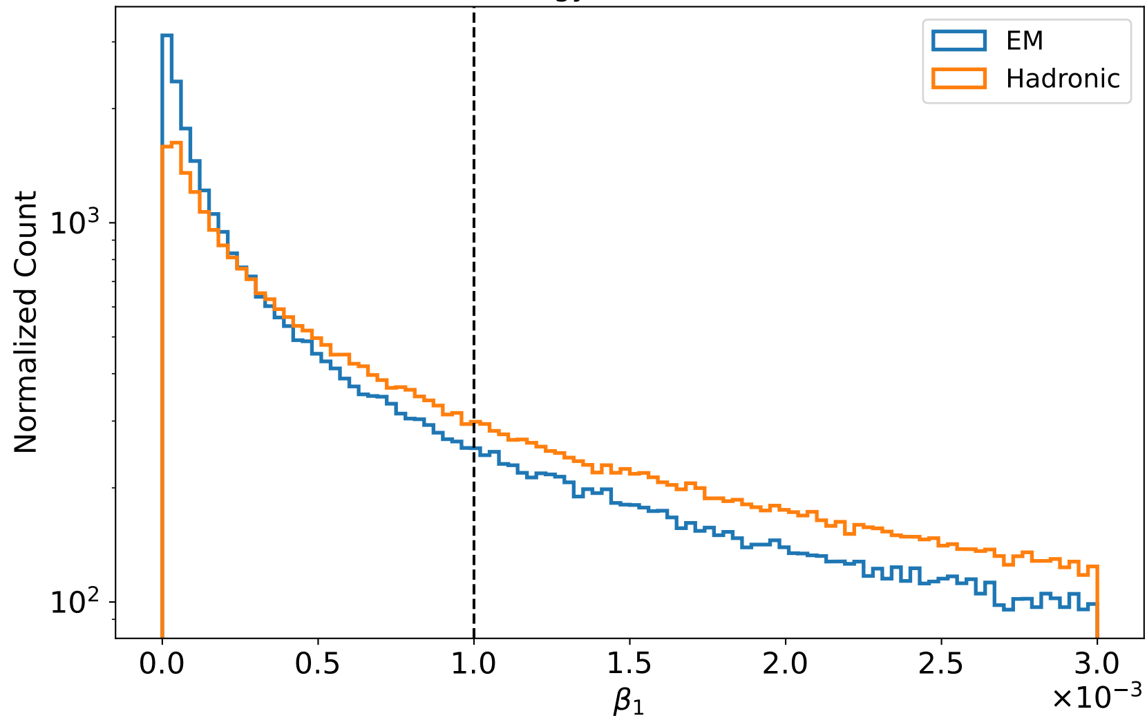
Energy 1 - 100 GeV
