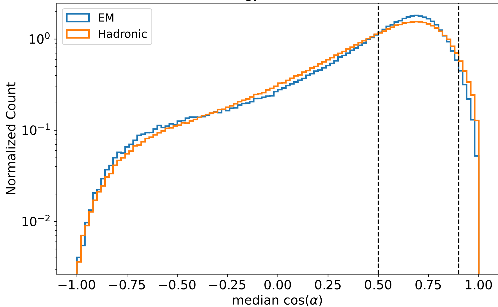
Energy 1 - 100 GeV
