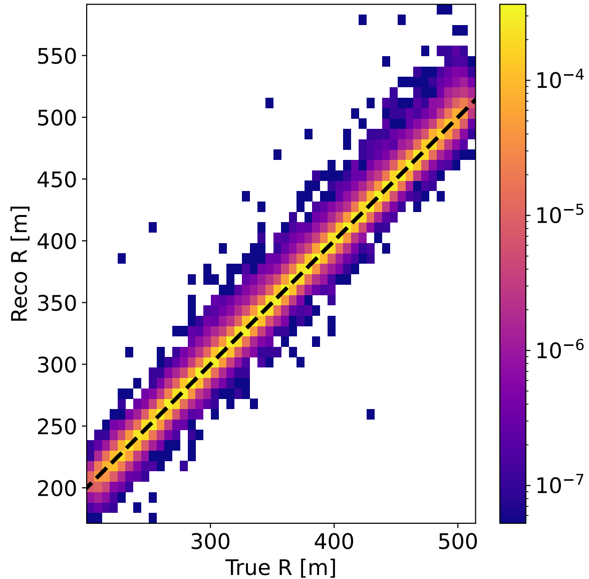
Hadronic
