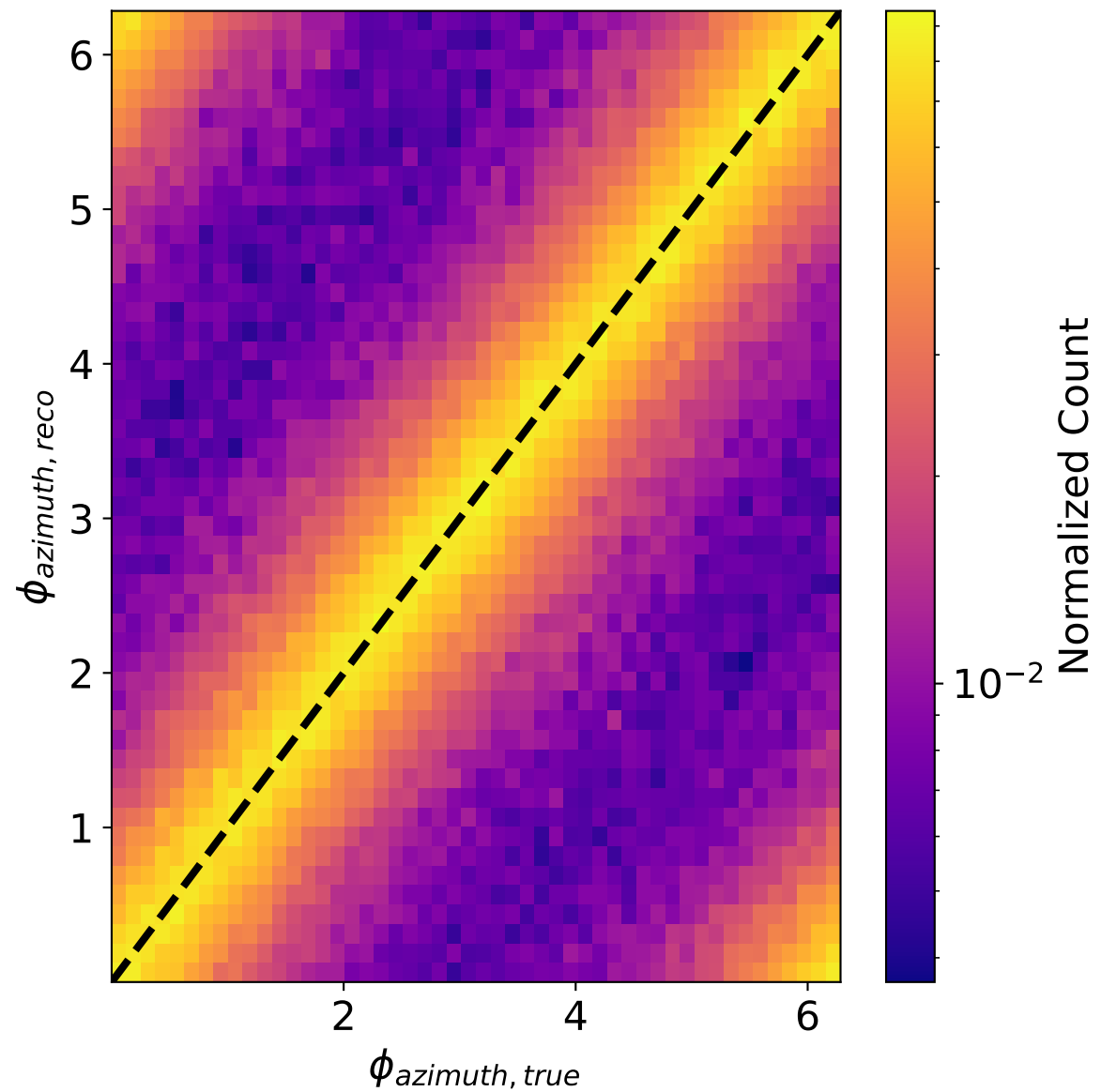
Hadronic
