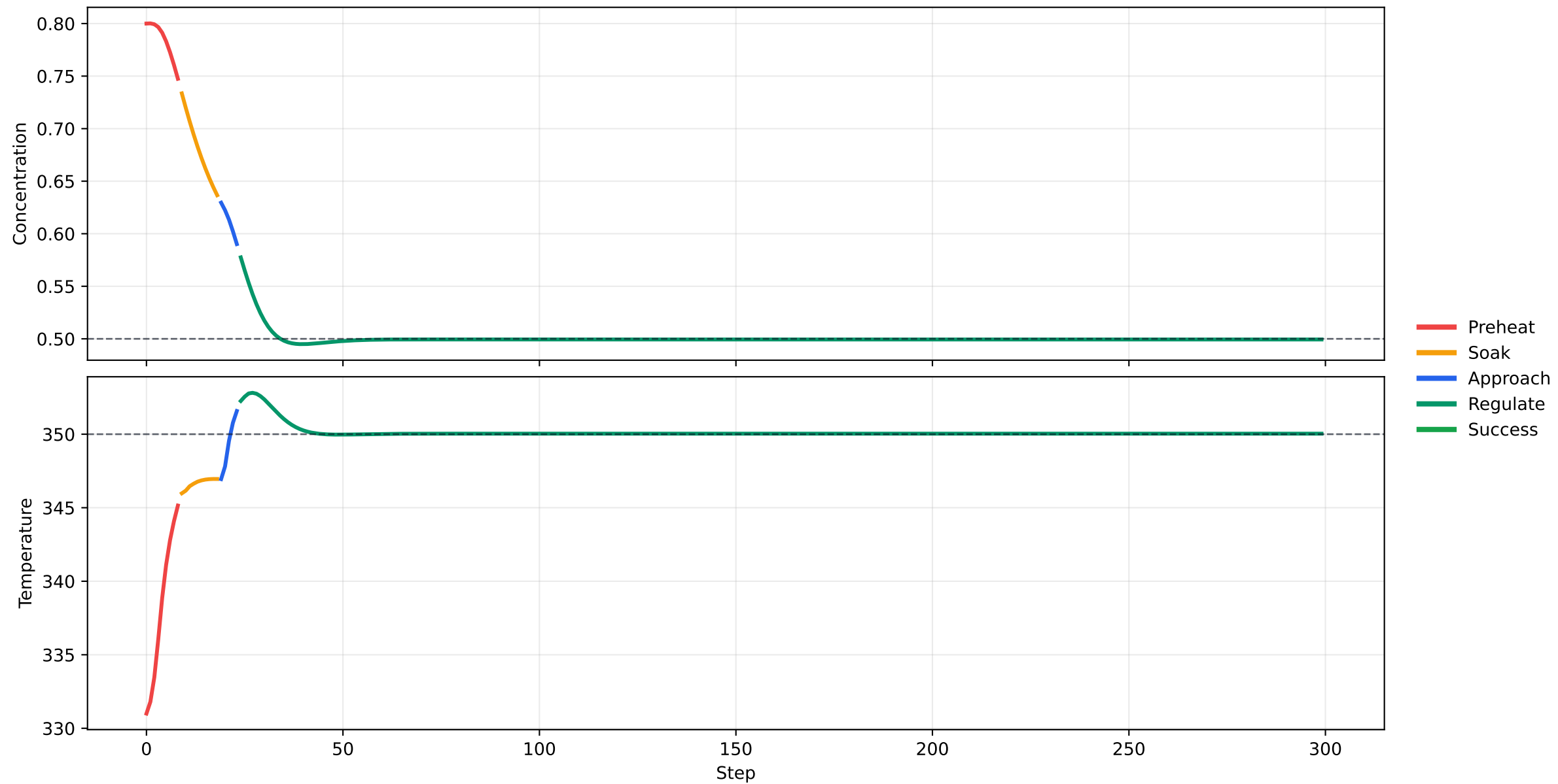
CSTR RML graph trajectory by protocol phase, seed 0
