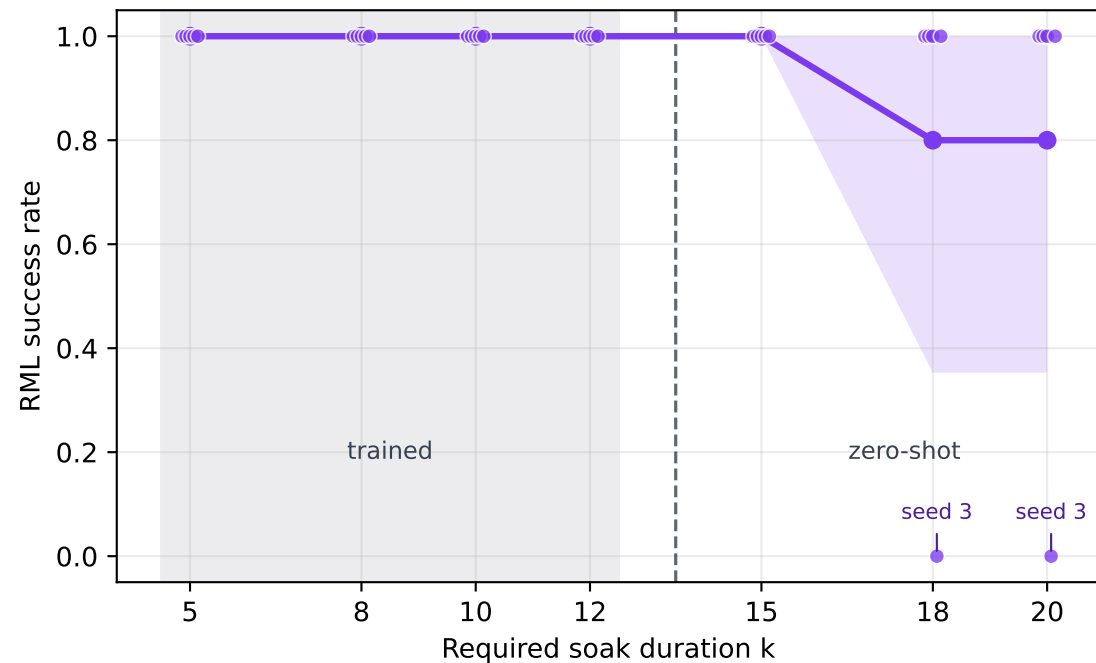
CSTR zero-shot soak generalization
