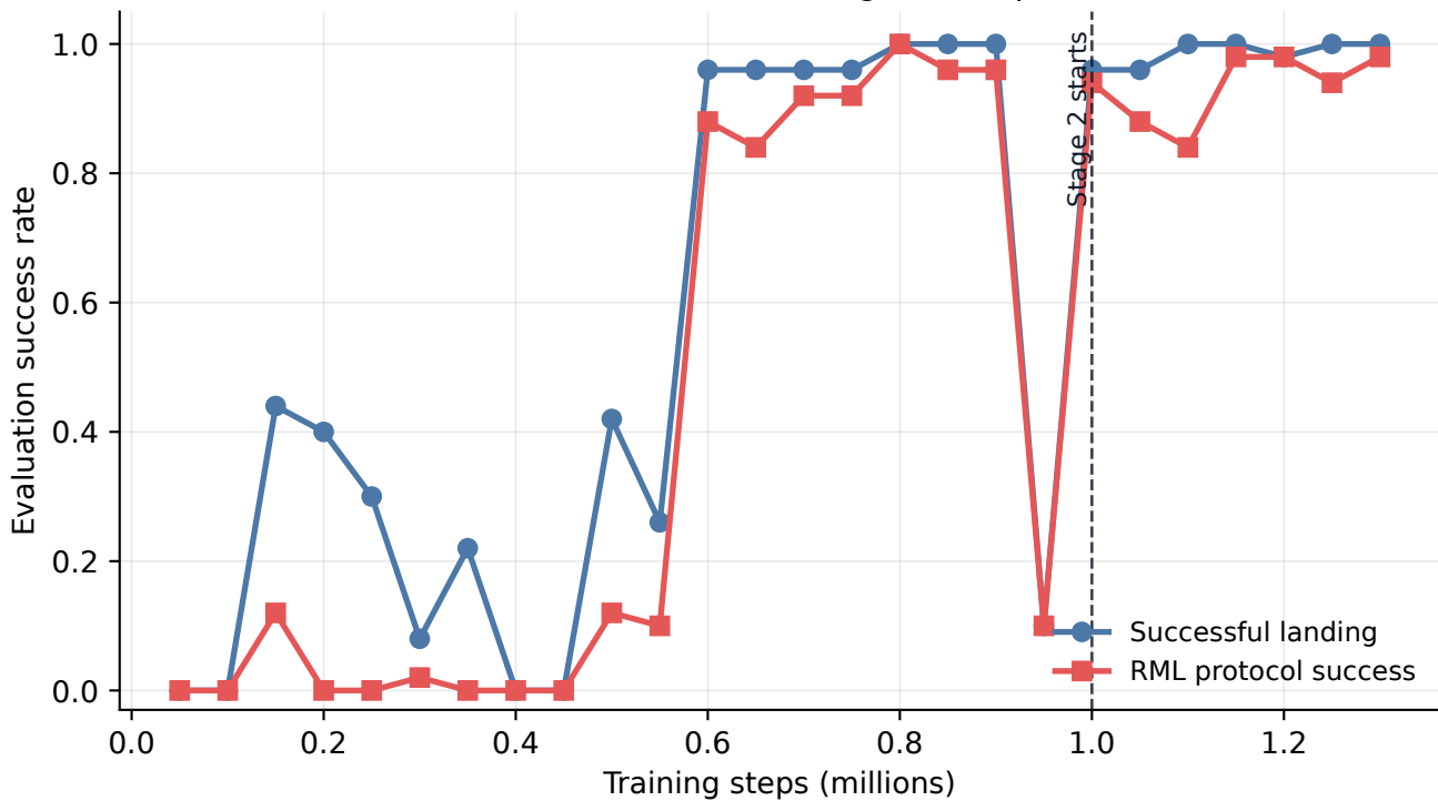
LunarLander seed 0: landing vs RML protocol
